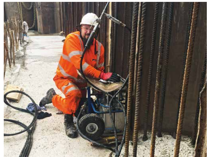
Sealing injection with ram injection lances between bored pile and sheet pile wall
